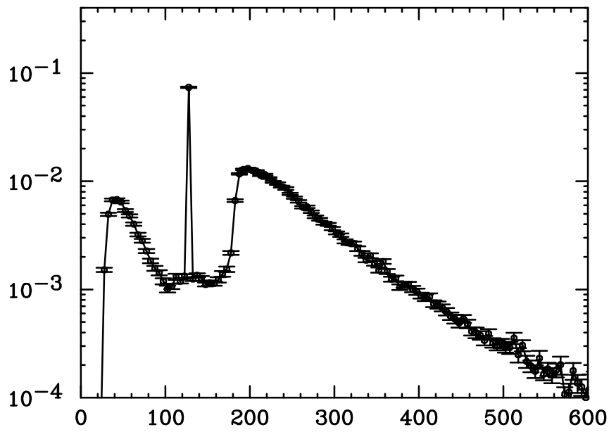
m4l distribution for 2l2l Higgs + gg continuum + interference
